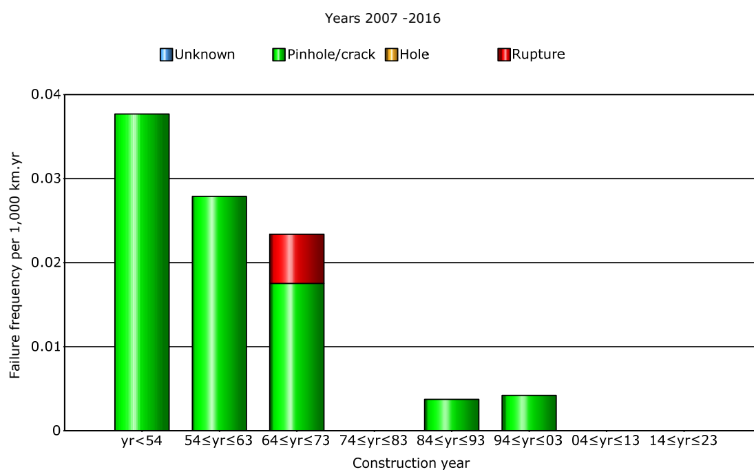
Figure 37: Relationship material failure, size of leak and year of construction (2007-2016)
