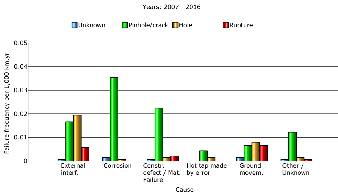
Figure 18: Relationship primary failure frequency, cause and size of leak (2007-2016)
